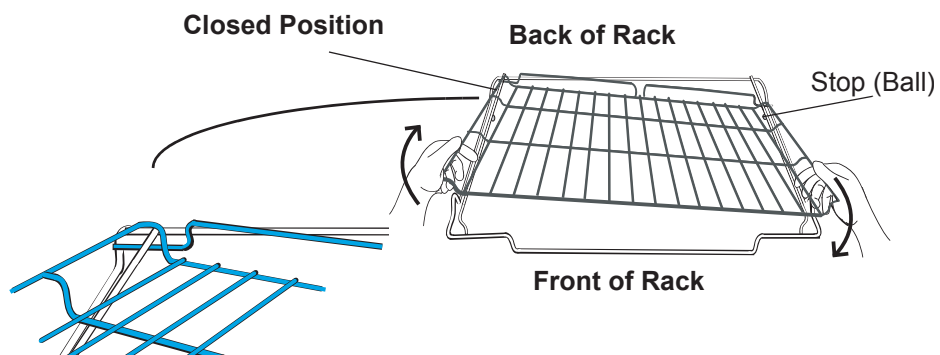
Figure 5: Disassembly
