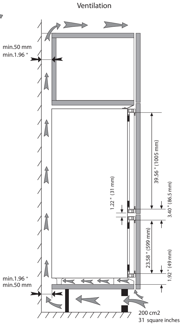
Ventilation requirement
