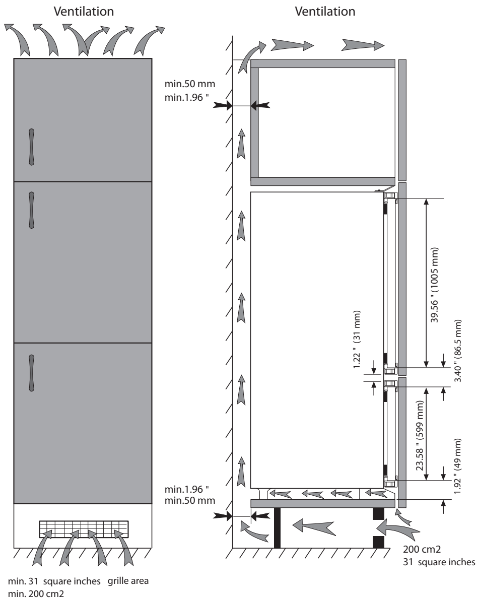
Ventilation requirement
