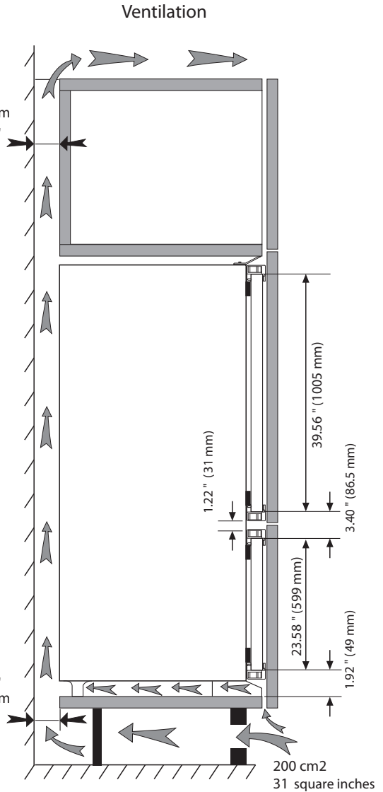
Ventilation requirement
