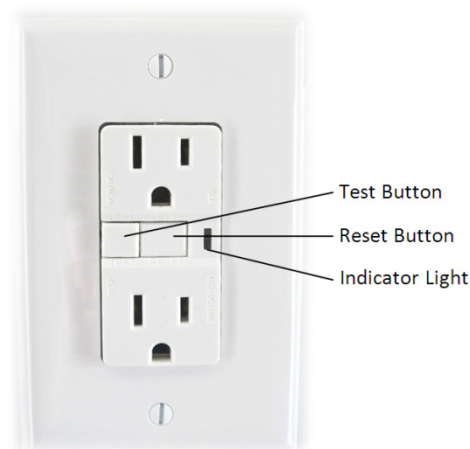
GFCI Outlet
