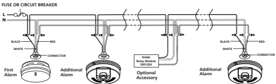
Interconnect Wiring Diagram
